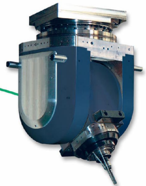
Direct drive 2-axis NC milling head (Opt.)
