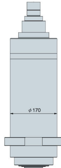
HSK A63 (for AC42)
